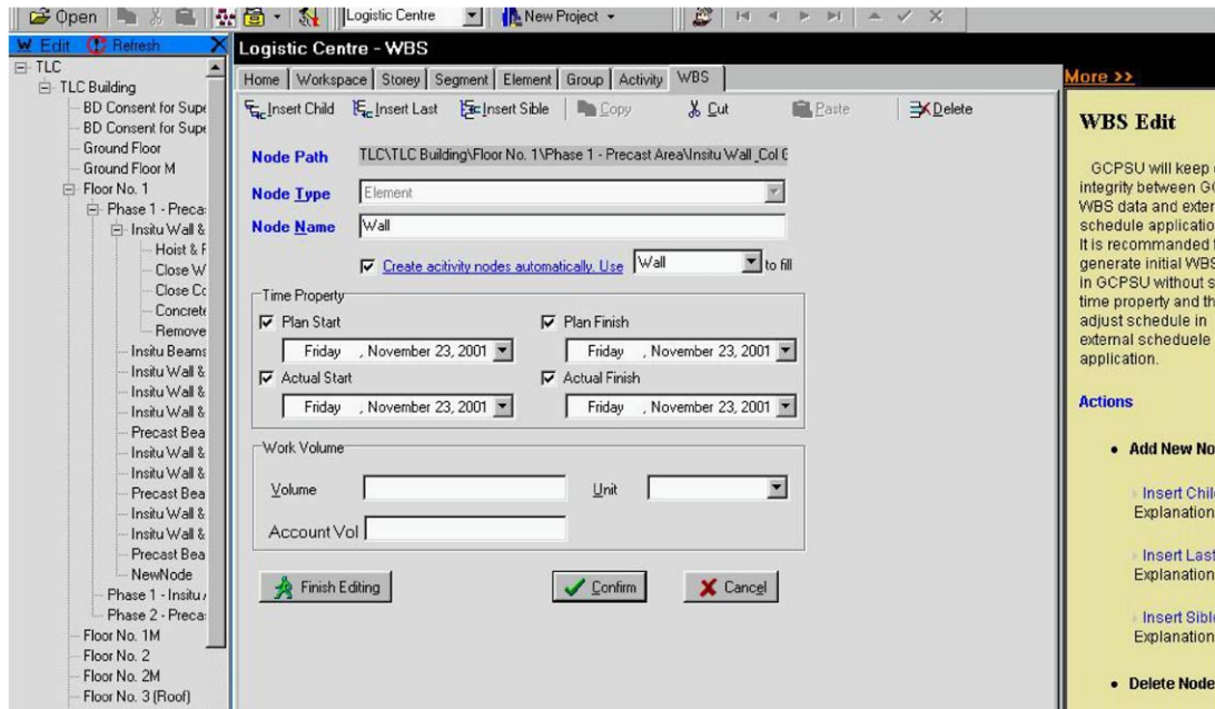
Fig. 6. WBS editor.
